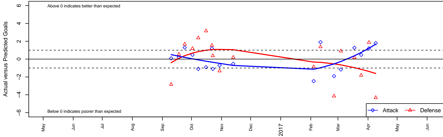
Highline Premier Heat Red B05 Dots are actual minus expected GF (blue circles) and GA (red triangles). Blue line is smoothed change in attack strength. Red is smoothed change in defense strength.
